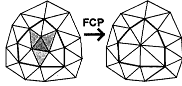
Figure 2: The Face Constriction Process. The dark-shadowed triangle is constricted into a new vertex. Its three adjacent triangles become degenerated and are deleted.
