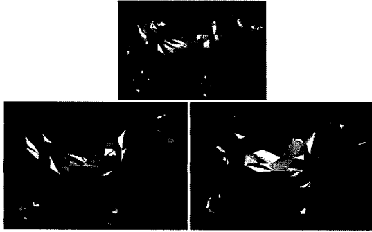
Figure 11: Comparison with Gieng et al's scheme. The original model of 5,804 faces (top), simplified models of 1,500 faces using our method (bottom-left) and Gieng et al's (bottom-right).
