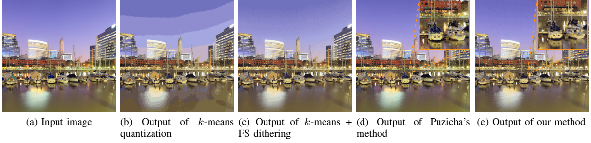
Fig. 1. Combined quantization and dithering to a palette of 32 colors. (a) Input image. (b) The result of k -means quantization; note the obvious false edge artifacts. (c) Using the same palette, Floyd-Steinberg dithering leads to fewer false edges. (d) The result of Puzicha's method, which preserves the original colors and suppresses false edges better than (c), but at the cost of greater noise. (e) The result of our combined quantization and dithering method, which preserves the original colors better, has fewer visible false edges, and largely suppresses noise.
