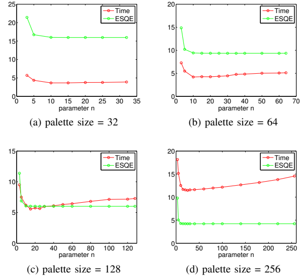
Fig. 4. The effect of parameter n . For palette size of 256, the fastest speed without sacrificing quality is achieved at about n = 25 . Similarly, n = 10, 10, 15 are best values for palette sizes of 32, 64 and 128, respectively.
