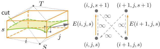
Figure 9: The local warping could be regarded as a continuous cut of the function E (left). The weights on edges are shown on the right. For simplicity, we show the forward edges (dashed lines) only in 2D. In general, forward edges are added in the s-x and s-y planes.
