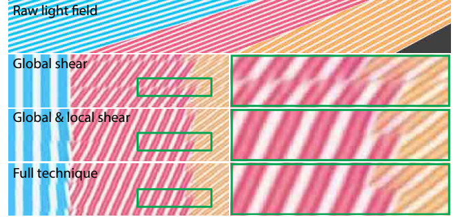
Figure 16: Results of our technique with certain steps omitted. The global shear of the original light field reduced excessive disparities and provided a good alignment of the blue lines. Local shearing significantly improved the discontinuities between the red lines. In this case, this is achieved by locally sacrificing the continuity of the blue lines, which does not influence significantly the overall quality across all views. The complete technique was able to match the red and yellow lines to further improve the continuity between the replicas. The Poisson reconstruction was applied in all examples.
