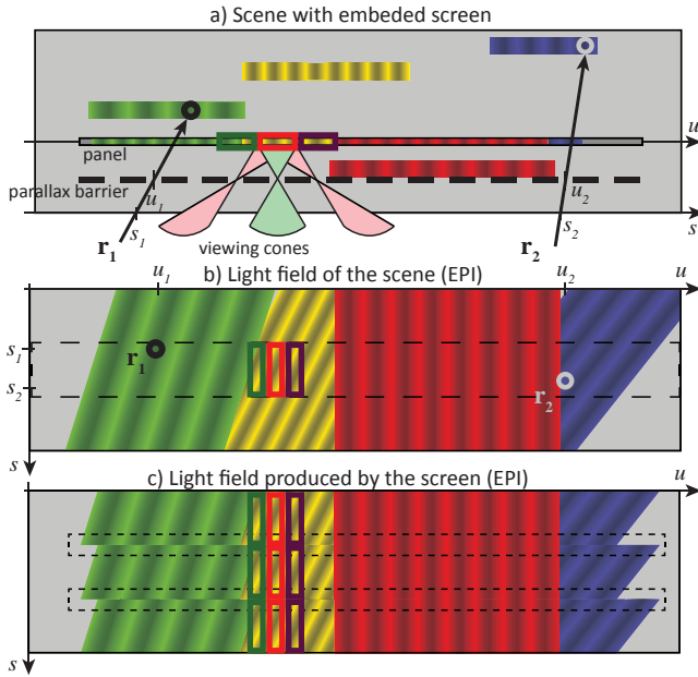
Figure 3: A simple scene (top) and the corresponding light field (middle). Rays r_1 and r_2 show the relationship between the scene and the light field representation. To visualize the relation between the scene light field and the light field produced by the display, we embedded the screen in the scene (top). For simplicity, we assumed its alignment with the u axis. The bottom image shows the light field that is produced by the display. Due to the limited angular coverage of the display with views (green cone), the screen is able to reproduce only a part of the original light field (marked with the dashed line in (b)). Beyond this range, the screen creates replicas of the light field, which results in discontinuities (dashed line in (c)).
