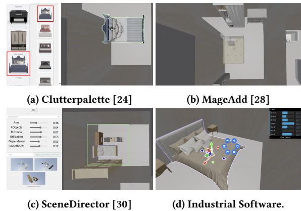
Figure 10: The four baselines in addition to our framework. (a): Clutterpalette [24] adds objects (Red Boxes) according to their surrounding contexts. (b): MageAdd [28] explores potential objects that can be added, e.g., the translucent object in the scene. (c): SceneDirector [30] edits multiple objects concurrently (Green Box). (d): Typical industrial solutions are integrated into our platform.
