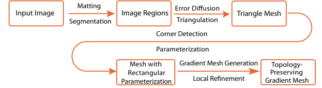
Figure 3: Algorithm pipeline.
