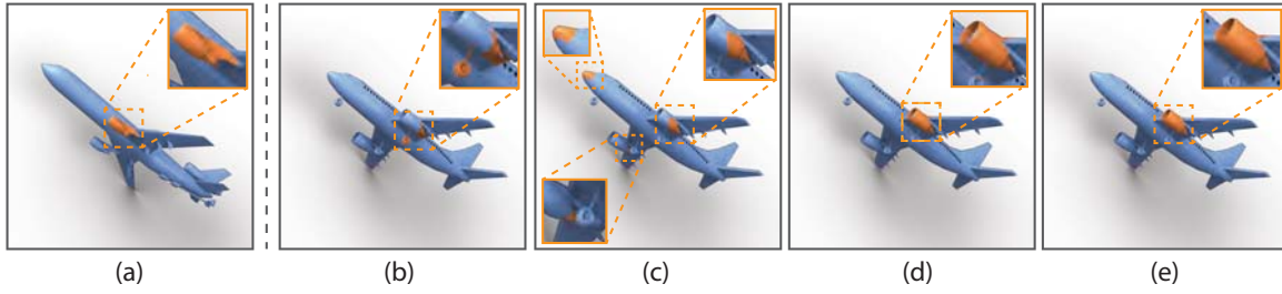
Fig. 6. An example demonstrating local correspondence. (a) an engine selected by the user from one model. (b-d) Corresponding regions in another model using thresholding of fuzzy correspondence response, with only geometric closeness (b), feature closeness (c) and both (d). (e) the final region after the MRF-based optimization.
