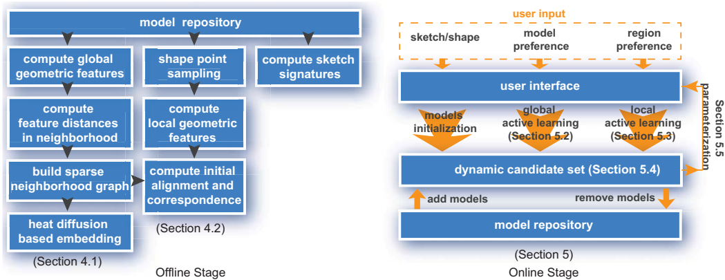
Fig. 2. System pipeline.
